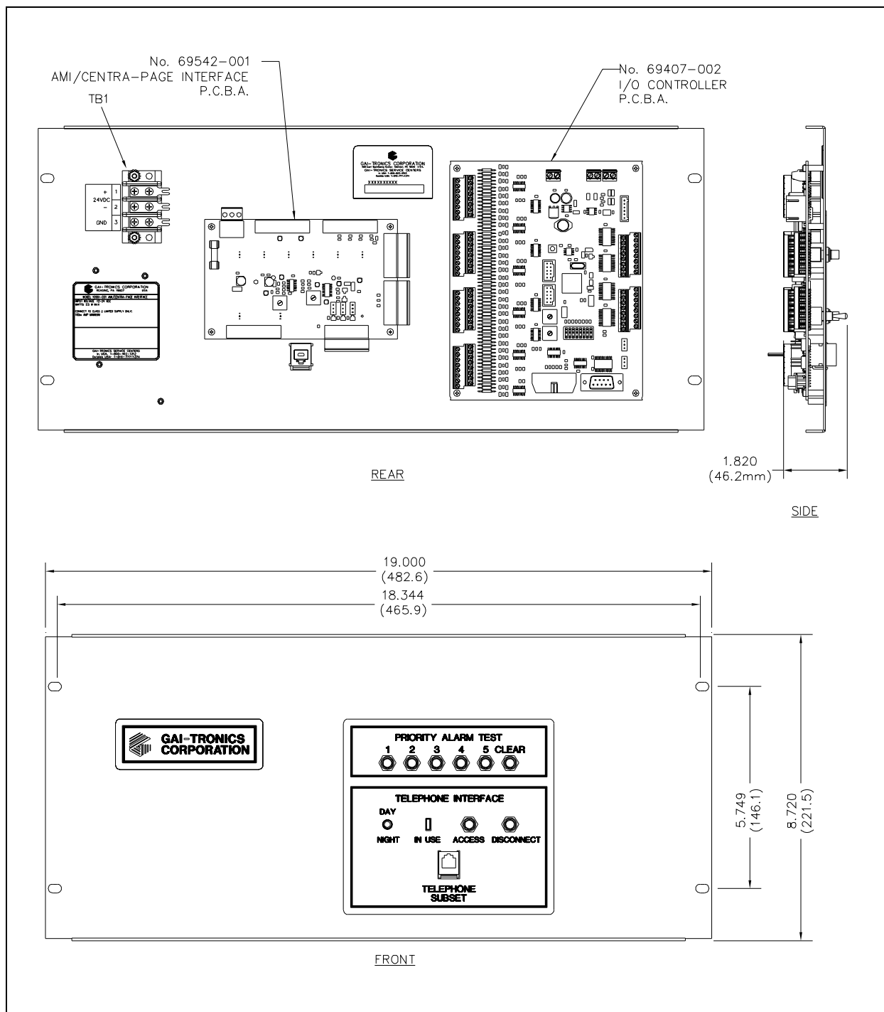
Figure 1. Model 10961-001 AMI Centra-Page Interface
