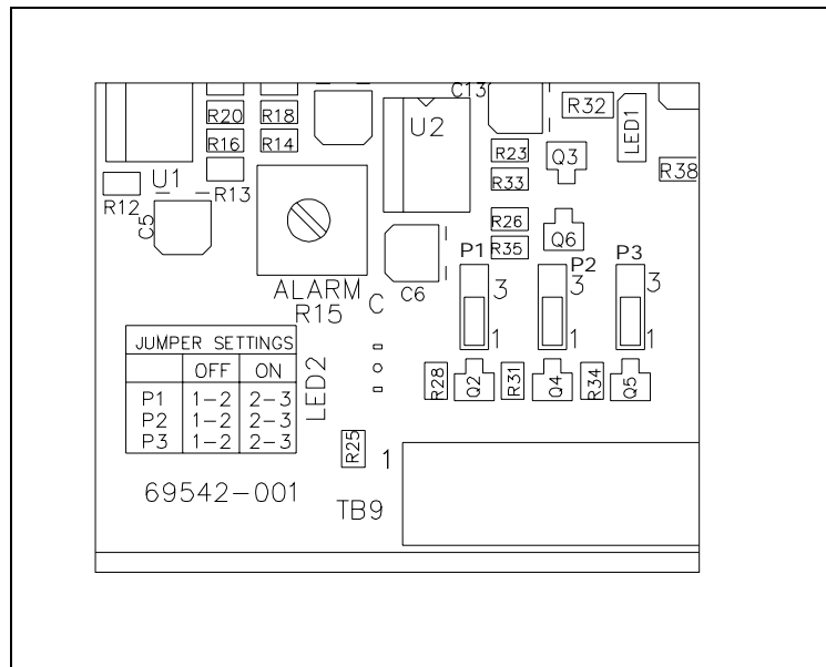
Figure 9. Crew's Quarters Jumpers on the 69542-001 PCBA in the Model 10961-001 AMI Centra-Page Interface
