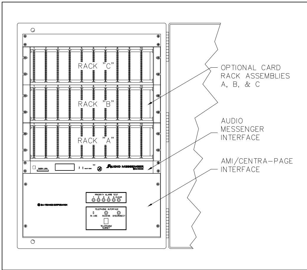
Figure 2. Centra-Page Central Cabinet with AMI and AMI Centra-Page Interface (front of center section)
